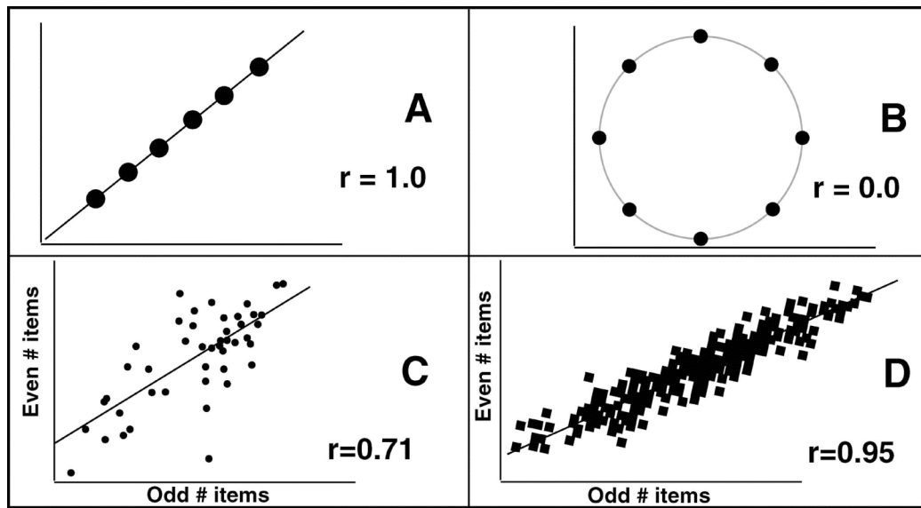
Figure 1. Scatter plots with associated correlation coefficients show predictability. “A” is a perfect correlation between two variables; r = 1.0 . It has perfect predictability of one variable when the other is measured. “B” is zero correlation. “C” is from test data in a freshman course that yields r = 0.71 . The scatter is apparent but the pattern is elongate. One can see by picking any individual point at random that predictability is only fair at best. “D” is from a knowledge survey data from nearly 300 freshmen. The scatter pattern is very elongate and yields an r -value of 0.95. Predictability for nearly all individuals is very good
