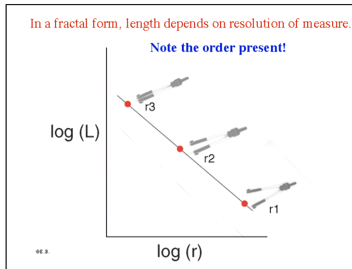
Figure 5. Understanding the coastline requires multiple measures, not just one. Note how the order of a fractal form becomes apparent as the coastal length changes almost in a perfectly predictable manner as the divider lengths are changed. This depiction of a fractal form was inspired by Benoit Mandelbrot's article in Science, 1967, "How long is the Coast of Britain?"
